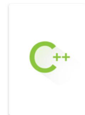
Native C++
